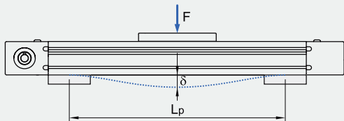
Fixed - fixed mounting
